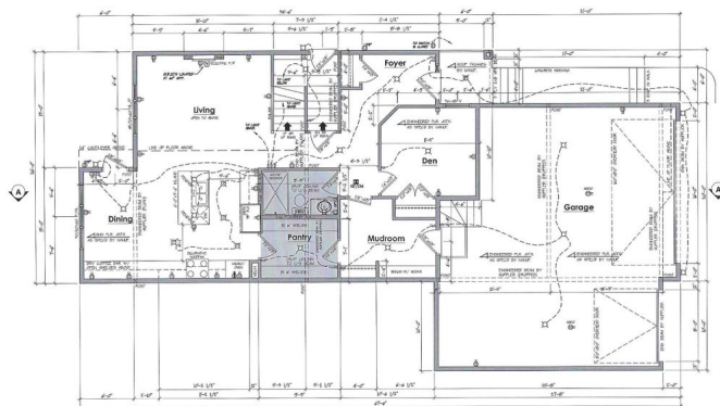
Main Floor Plan
